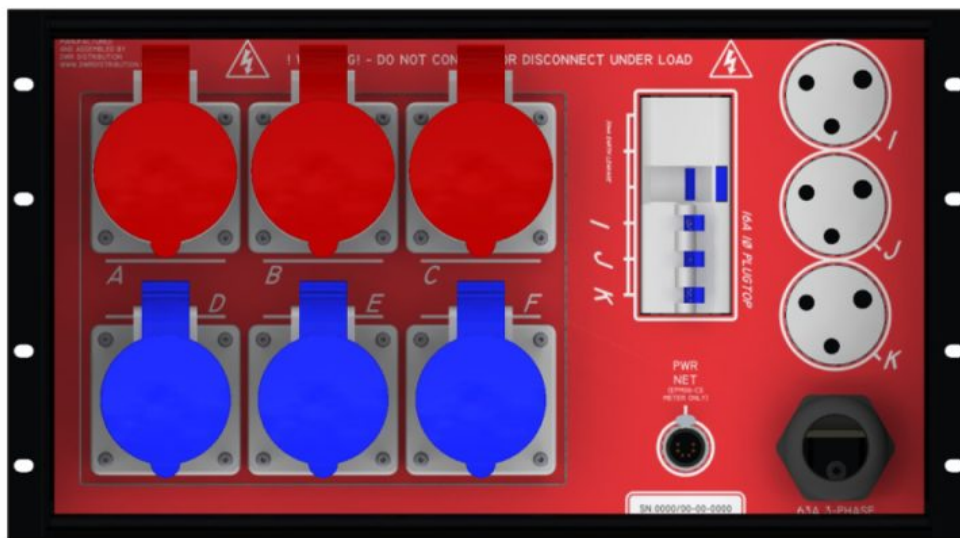
REAR VIEW
