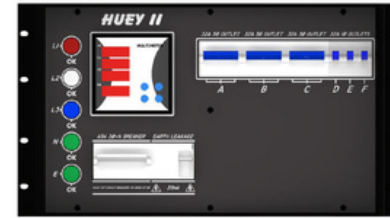
HUEY II 63A 3-PHASE
